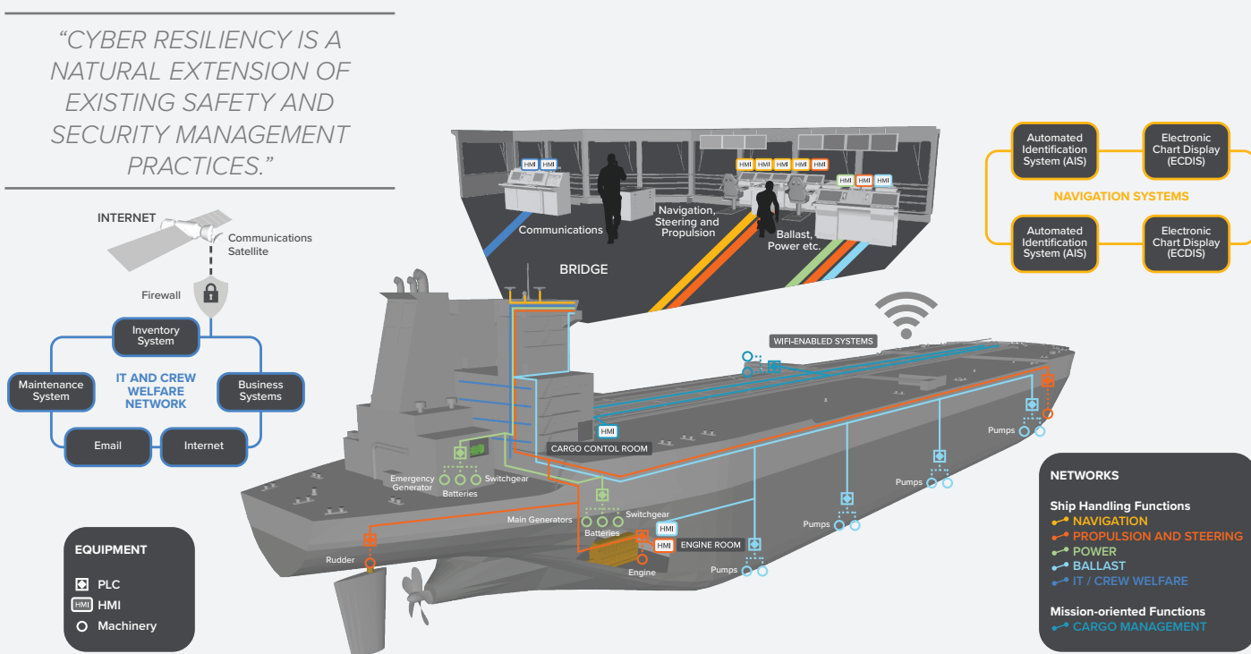
Figure 3 – Vulnerable OT assets increasingly exposed to cyber risk include navigation, propulsion, access control, management and communication systems.
